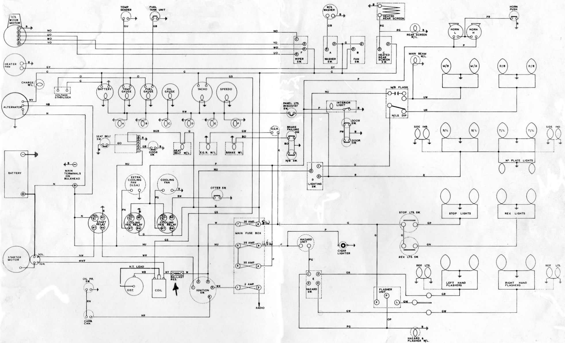
Theoretical Circuit Diagram for TVR "M" Series from Chassis No. 3668
